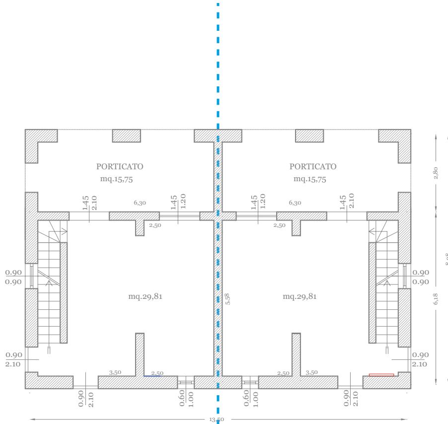
Hilltop House Nr 3A Ground Floor
