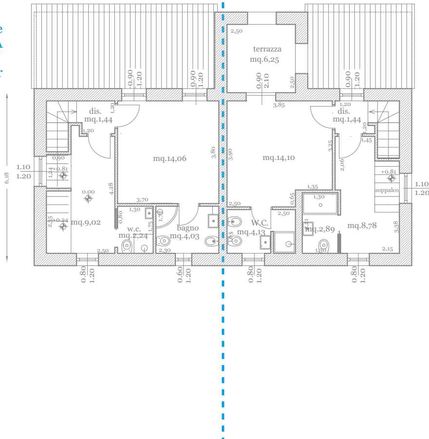
Hilltop House Nr 3A First Floor
